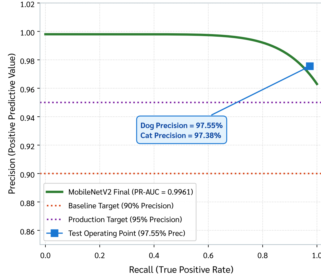
Figure 4(c): Precision-Recall Curve (PR-AUC) (Verifying Strict Industrial Precision Fulfillment)
