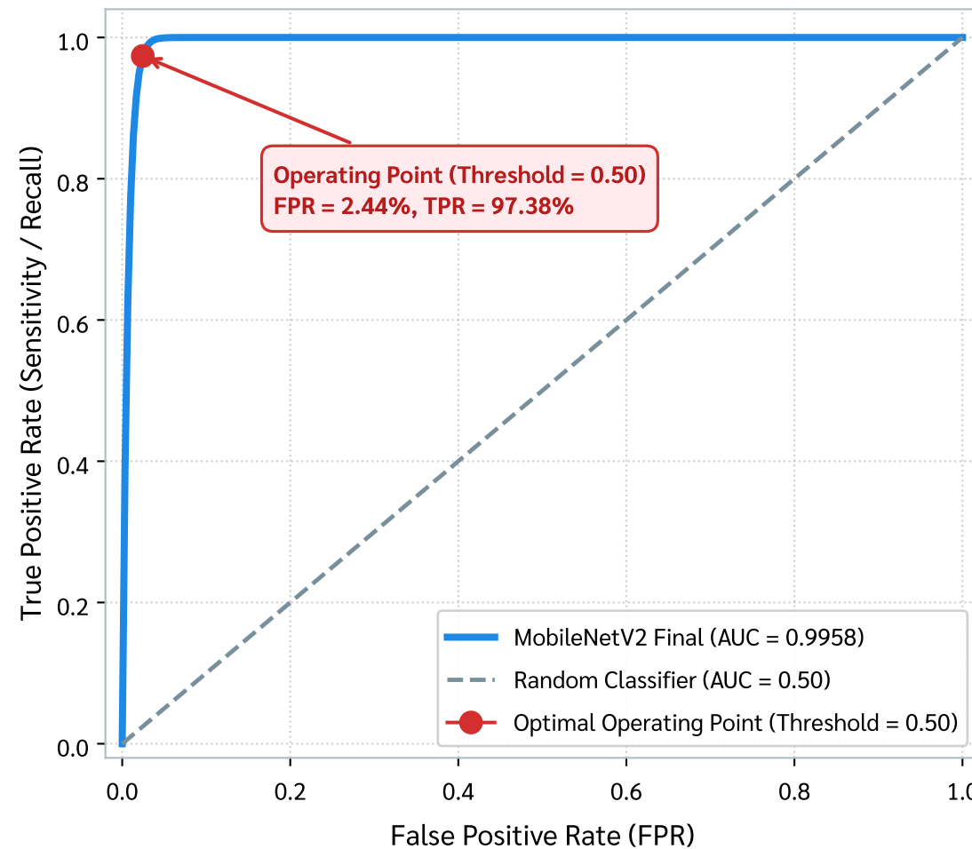
Figure 4(b): Receiver Operating Characteristic (ROC) (Confirming Near-Perfect Class Discrimination)
