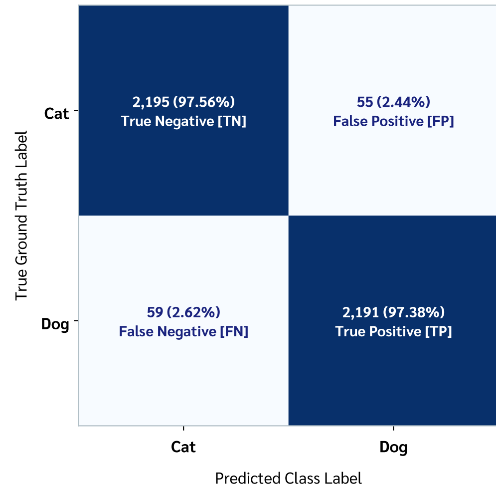
Figure 4(a): Normalized Confusion Matrix (Validation Holdout Set, N = 4,500 Images)
